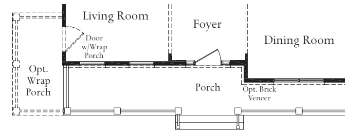
Partial main level with elev. 2
